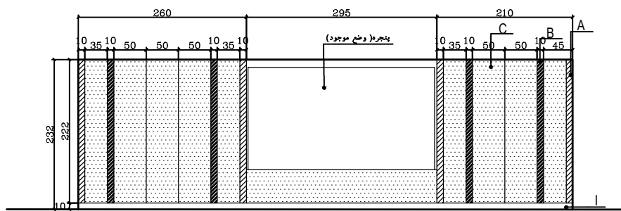
VIEW-A SCALE 1:20
