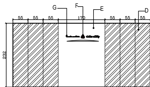
VIEW-C SC 1:20
